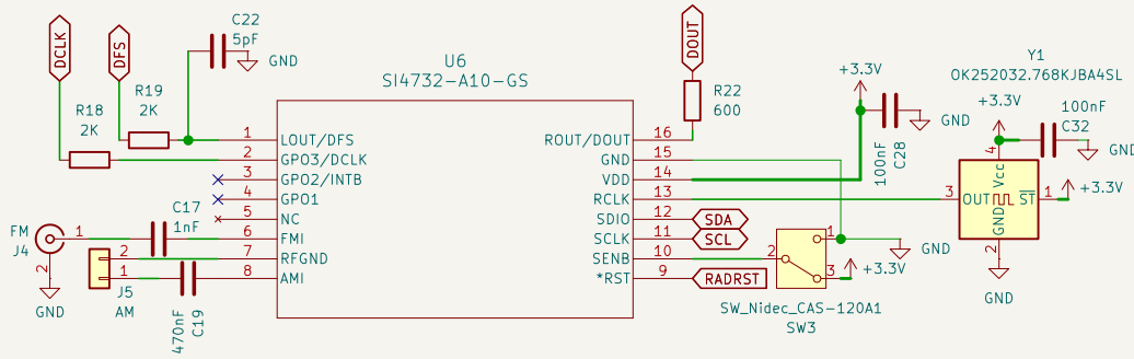
Si4732 AM/FM Radio
