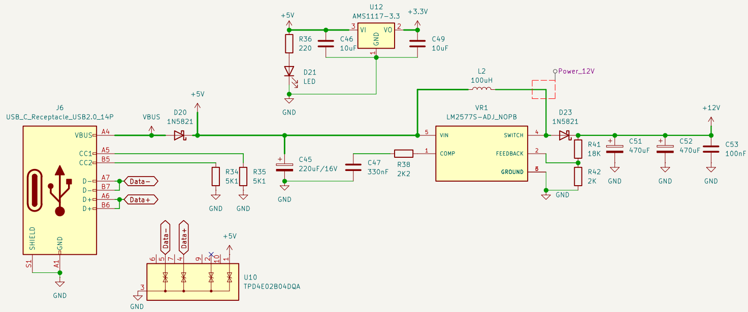
USB Type C 3.3/5/12V PSU
