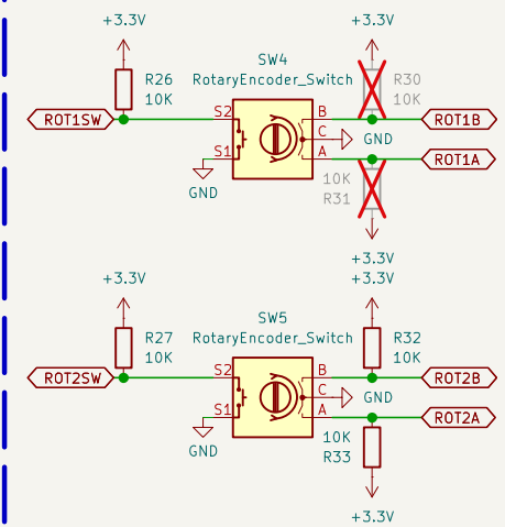
Rotary Encoders
