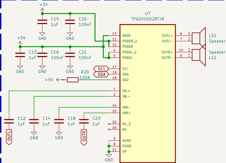
TPA2016 Dual Channel Amplifier
