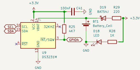
DS3231 RTC Clock
