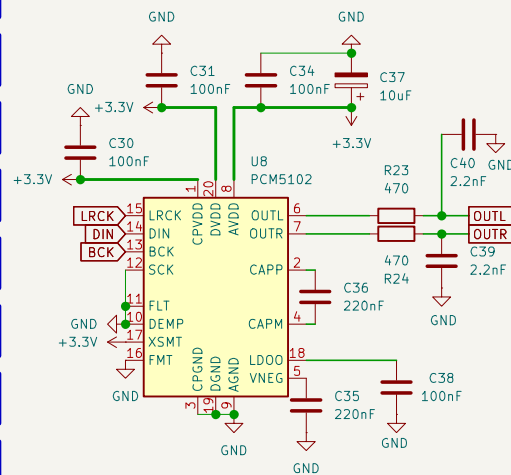
PCM5102 DAC
